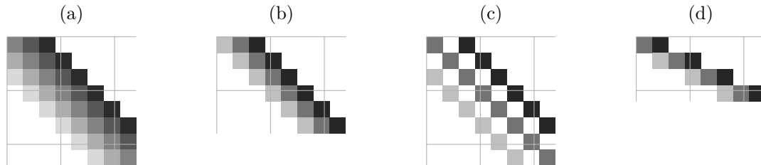
Figure 28: Weight matrices \Omega of four one-dimensional convolutional layers with eight inputs (columns) and one row per output; shading marks the kernel weights \omega_1, \omega_2, \dots from light to dark, white entries are zero. (a) Kernel size 5, stride 1, dilation 1, zero padding. (b) Kernel size 3, stride 1, dilation 1, valid (six outputs). (c) Kernel size 3, stride 1, dilation 2, zero padding. (d) Kernel size 3, stride 2, dilation 1, zero padding (four outputs).
