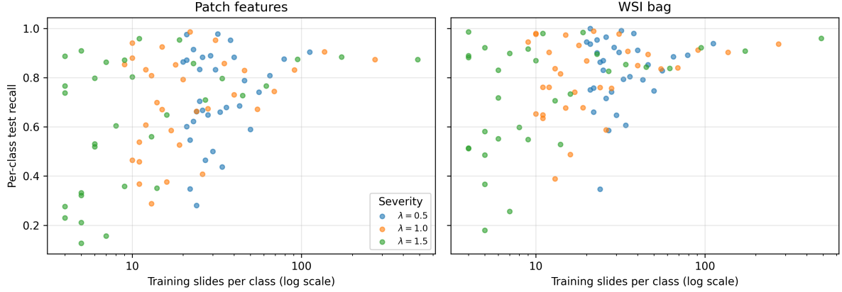
Figure 2: Per-class test recall against training slides per class (log scale), one panel per regime. Each point is a cancer type at one severity, averaged over methods and seeds; colour encodes the imbalance parameter \lambda . The horizontal axis is log-scaled.
