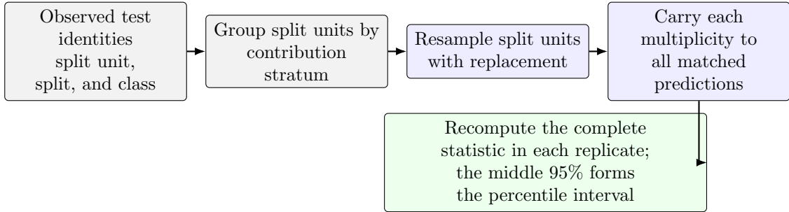
Figure 5: Split-unit-clustered bootstrap workflow. The label-only preflight executes the identity, stratification, and resampling steps before predictions exist. After model fitting, the same paired multiplicities are applied to every matched run.
