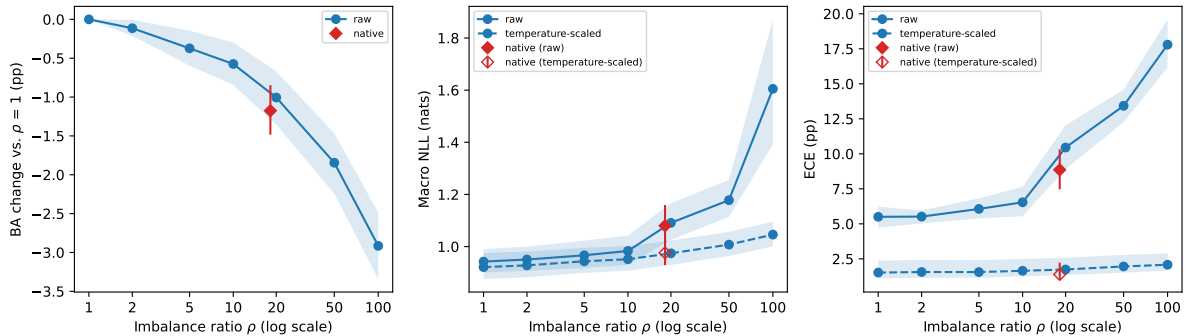
Figure 1: Balanced accuracy degrades slowly and accelerates beyond \rho = 10 ; raw calibration degrades much faster but recovers almost completely under temperature scaling. Blue lines connect the ratio arms at their realized ratio, with shaded paired 95% bootstrap bands; the red diamonds mark the native allocation at its realized ratio of 18.1. Left: change in patient-macro balanced accuracy relative to the balanced arm. Middle and right: macro NLL and ECE, raw (solid, filled) and after validation temperature scaling (dashed, open).
