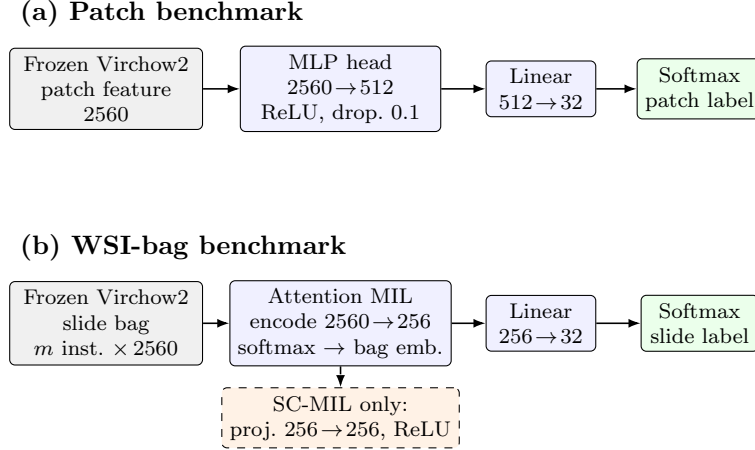
Figure 3: Shared classifier heads for the benchmark. Panel (a) classifies one controlled patch embedding per forward pass. CFAL reuses the MLP trunk but replaces the linear 512 \rightarrow 32 head with learnable prototypes and affinity-based prediction. Panel (b) encodes all instances on a slide, pools them with attention, and predicts one slide-level label; the dashed branch is used only by SC-MIL. MDE-MIL reuses the same attention trunk but replaces the single linear head with two expert heads and mean-logit ensemble inference at evaluation. Virchow2 features are frozen in both benchmarks.
