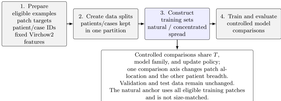
Figure 1: Controlled benchmark design. Gray boxes define shared evidence, partitioning, and evaluation; the blue box contains the training-support intervention.
