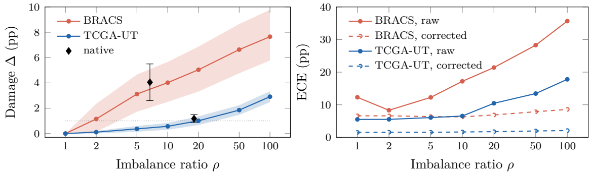
Figure 2: Left: balanced-accuracy damage versus \rho with 95% bands; diamonds mark native class shares, dotted line the 1-pp threshold. Right: expected calibration error (ECE) of the raw predicted probabilities (solid) and after a single global confidence correction fitted on validation data (dashed).
