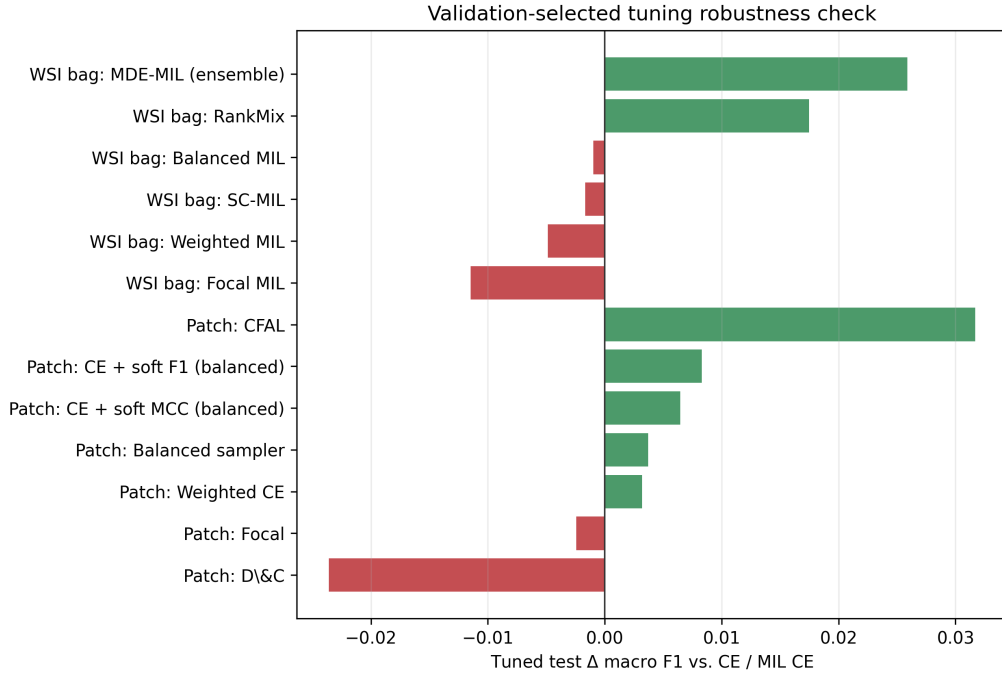
Figure 7: Held-out test macro-F1 change of secondary validation-selected configurations relative to the prespecified CE or MIL CE primary baseline.
