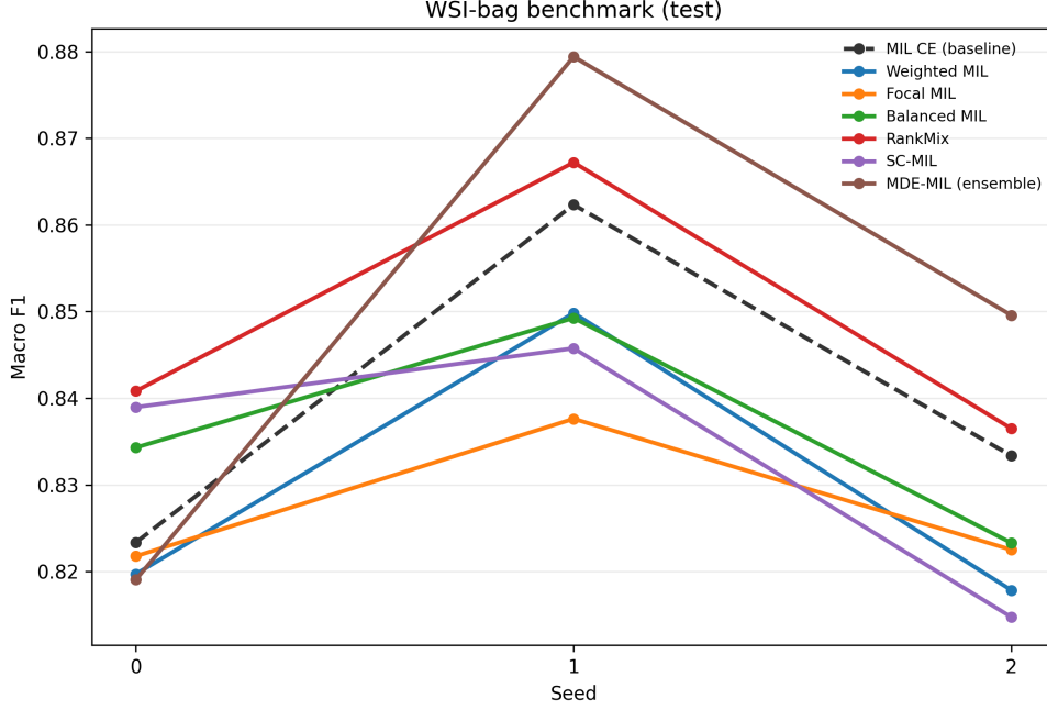
Figure 9: Primary-protocol WSI-bag macro F1 on the held-out test split by random seed. The dashed line marks plain MIL CE; seed-wise spread shows why cross-method gaps should be read cautiously when standard deviations overlap (Table 7).
