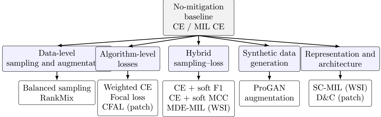
Figure 2: Method organization used in the benchmark. Cross-entropy is the no-mitigation reference, while the tested alternatives intervene through sampling, loss design, synthetic data, WSI feature augmentation, or representation learning.
