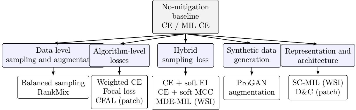
Figure 2: Method organization used in the benchmark. Cross-entropy is the no-mitigation reference, while the tested alternatives intervene through sampling, loss design, synthetic data, WSI feature augmentation, or representation learning.
