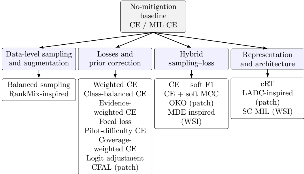
Figure 1: Intervention-level organization of the tested methods. Cross-entropy is the no-mitigation reference; alternatives intervene through sampling, objectives, prior correction, feature mixing, feature synthesis, or representation and classifier design. Table 2 adds the orthogonal signal axis.
