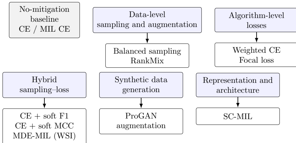
Figure 2: Method organization used in the benchmark. Cross-entropy is the no-mitigation reference, while the tested alternatives intervene through sampling, loss design, synthetic data, WSI feature augmentation, or representation learning.
