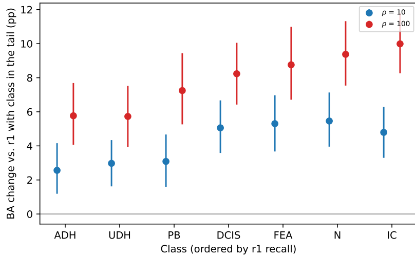
Figure 1: Easy classes cost the most when they sit in the tail. Balanced-accuracy loss against the balanced arm, in points, with the class on the horizontal axis placed in the tail, at \rho = 10 (blue) and \rho = 100 (red), with paired 95% bootstrap intervals. Classes are ordered by their recall in the balanced arm, from ADH (12 percent) to IC (69 percent).
