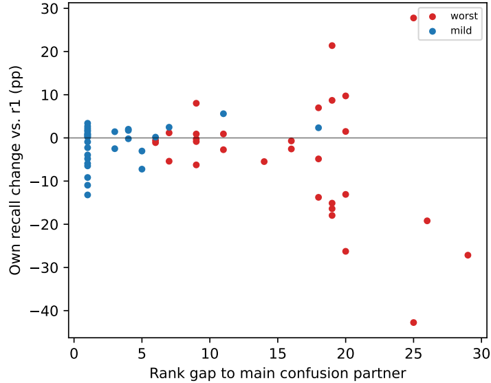
Figure 3: Recall changes spread widely only when a class is far in rank from its main confusion partner. Each point is one class under the worst (red) or mild (blue) order: the rank gap to the class it is most often predicted as in the balanced arm, against the pooled change in its own recall against r1.
