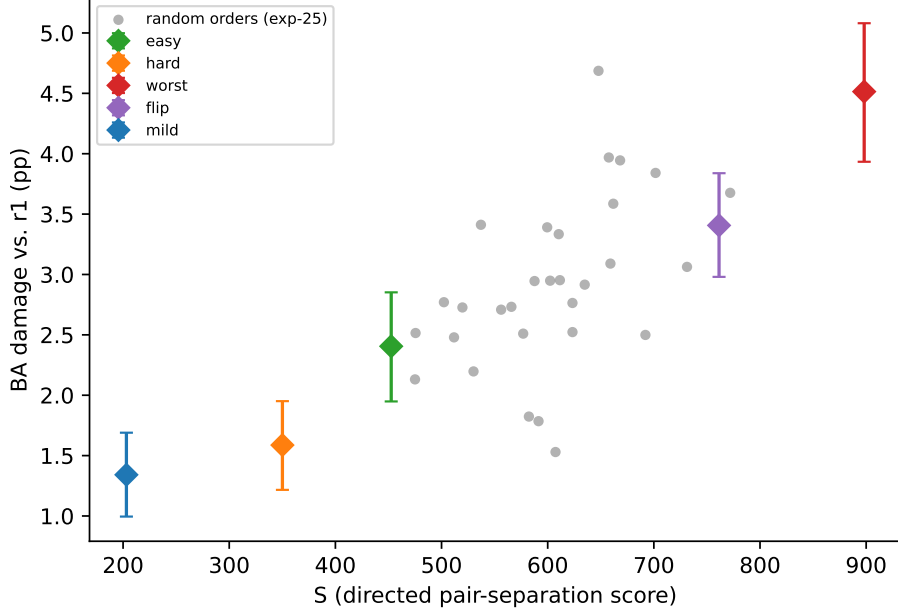
Figure 2: The derived orders extend the random-order trend in both directions. Observed balanced-accuracy damage against the rate-weighted score at \rho = 100 . Grey points: the 30 random class orders of the prevalence curve, one per fit. Diamonds with 95 percent bootstrap intervals, each pooled over 30 fits: hard-tail (orange) and easy-tail (green) orders of the tail-assignment study, and the mild (blue), flip (purple) and worst (red) orders fitted here.
