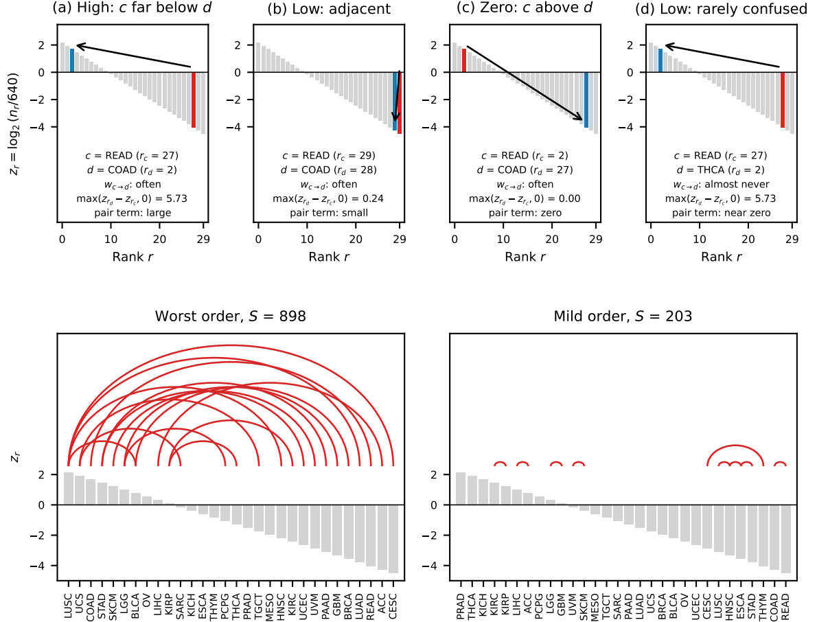
Figure 1: A pair term is large only when a frequently confused class sits far below its confusion partner, and the worst order stacks many such terms. Grey bars: log allocation z_r of each rank at \rho = 100 ; positive z_r means more than the balanced 640 patches, negative z_r fewer. Top, (a) to (d) from left to right: one term w_{c \rightarrow d} h_c \max(z_{r_d} - z_{r_c}, 0) of Equation (1), with class c in red and class d in blue; the arrow points from c to d . Bottom: the worst and mild orders, with class codes under their ranks. Each arc links a class to the class it is most often predicted as in the balanced arm and is drawn only when the class sits below that partner, that is, when its term is positive. Arcs show only the main partner of each class, whereas S sums over all pairs.
