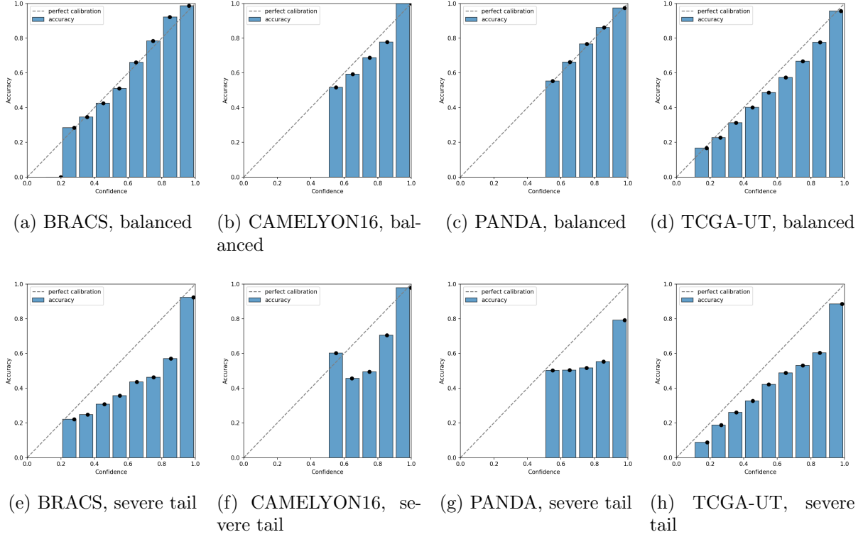
Figure 2: Reliability curves for the balanced reference and for the tail classes under the severe condition of the native assignment, with bin accuracy against mean predicted confidence over ten equal-width bins, on the first locked partition.
