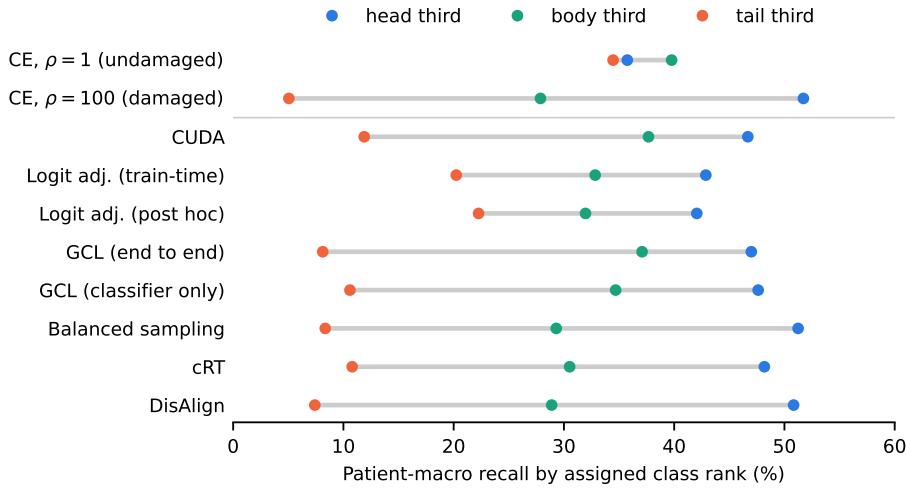
Figure 2: Only logit adjustment lifts tail recall substantially at \rho = 100 ; CUDA and GCL gain in the body, the other methods stay close to CE. Patient-macro recall of the head, body, and tail thirds of classes by assigned rank, averaged over shards.
