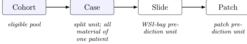
Figure 2: Nesting of the units evidence is counted in. Splits are drawn over cases, so slides and patches beneath one case are correlated rather than independent observations of its class.
