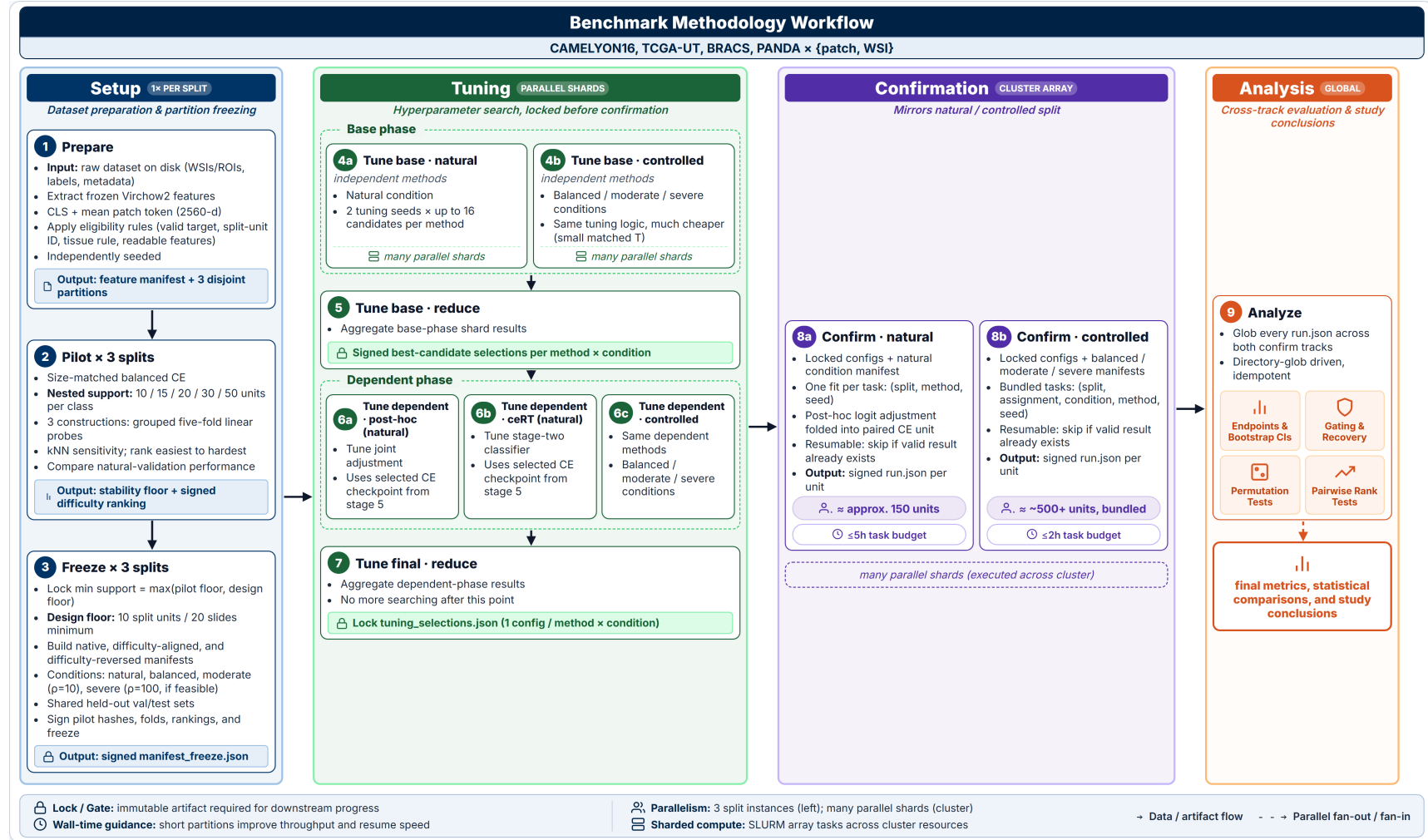
Figure 7: Operational workflow of the controlled class-imbalance benchmark.
