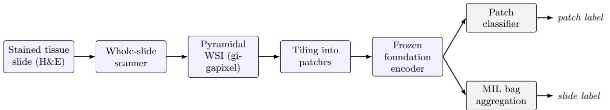
Figure 1: The computational-pathology pipeline used throughout the benchmarks. A stained slide is scanned into a pyramidal WSI and tiled into patches; a frozen foundation-model encoder embeds each patch once, after which either a patch classifier predicts a per-tile label or a multiple-instance head aggregates the patch features of a slide into a slide-level prediction.
