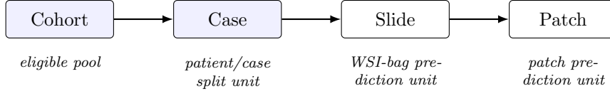
Figure 2: Nesting of the units independent support is counted in. Splits are drawn over cases, so slides and patches beneath one case are correlated rather than independent observations of its class.
