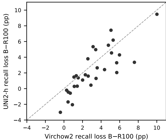
TCGA-UT
