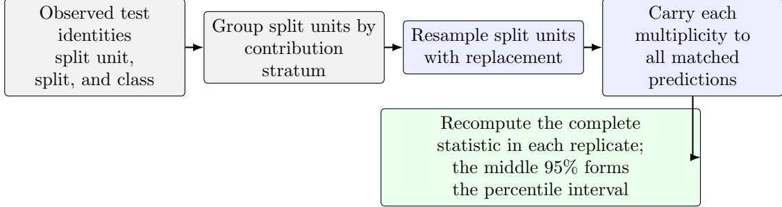
Figure 5: Split-unit-clustered bootstrap workflow. The label-only preflight executes the identity, stratification, and resampling steps before predictions exist. After model fitting, the same paired multiplicities are applied to every matched run.
