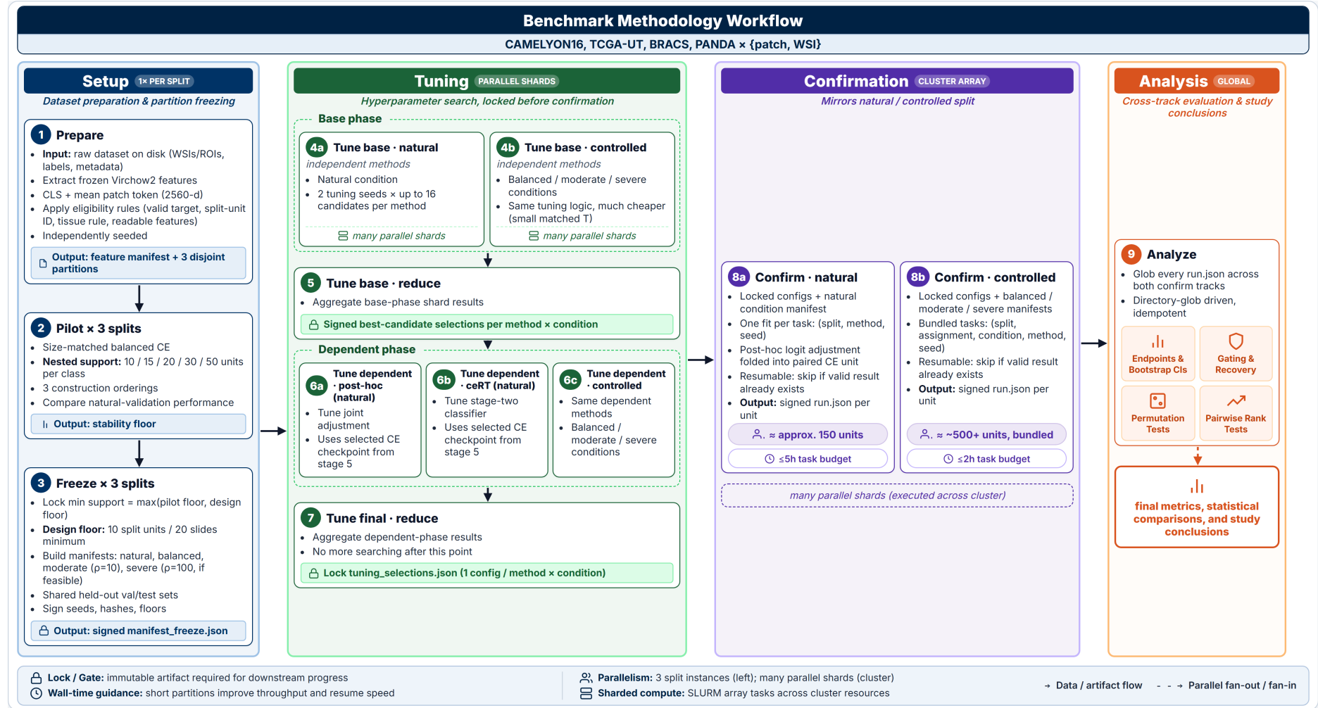
Figure 6: Overview of the controlled class-imbalance benchmark.
