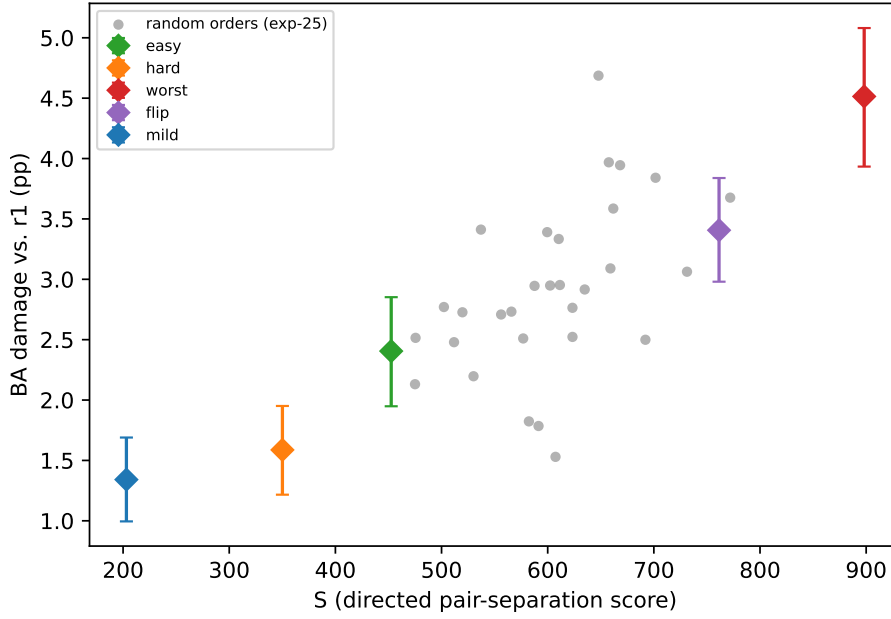
Figure 1: The derived orders extend the random-order trend in both directions. Observed balanced-accuracy damage against the rate-weighted score at \rho = 100 . Grey points: the 30 random class orders of the prevalence curve, one per fit. Diamonds with 95 percent bootstrap intervals, each pooled over 30 fits: hard-tail (orange) and easy-tail (green) orders of the tail-assignment study, and the mild (blue), flip (purple) and worst (red) orders fitted here.
