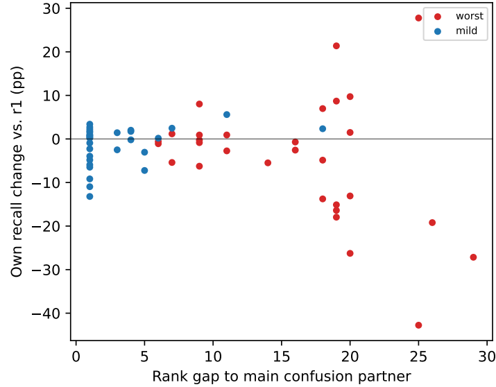
Figure 2: Recall changes spread widely only when a class is far in rank from its main confusion partner. Each point is one class under the worst (red) or mild (blue) order: the rank gap to the class it is most often predicted as in the balanced arm, against the pooled change in its own recall against r1.
