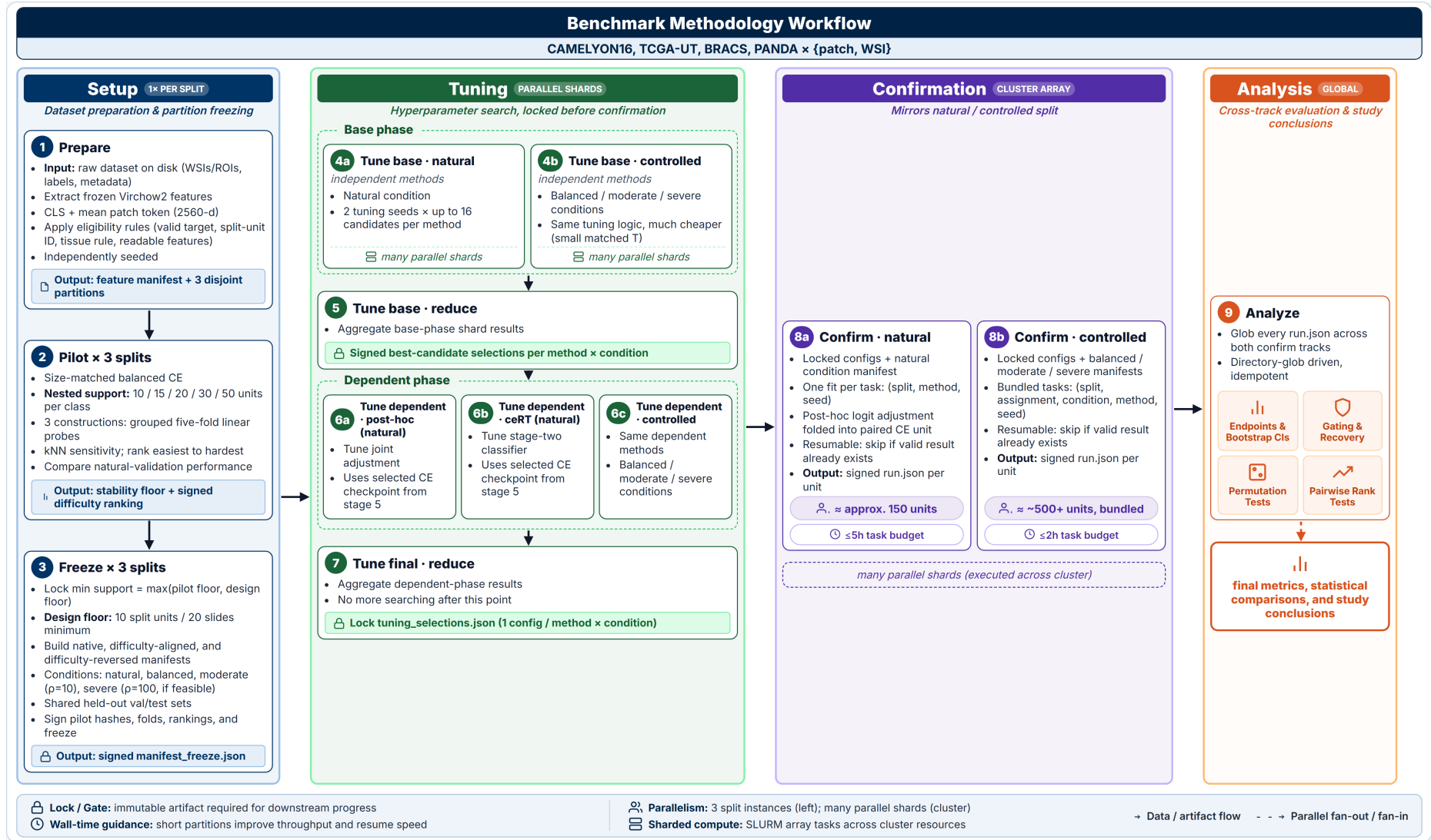
Figure 7: Operational workflow of the controlled class-imbalance benchmark, including immutable artifacts, parallel tuning, confirmation, and analysis.
