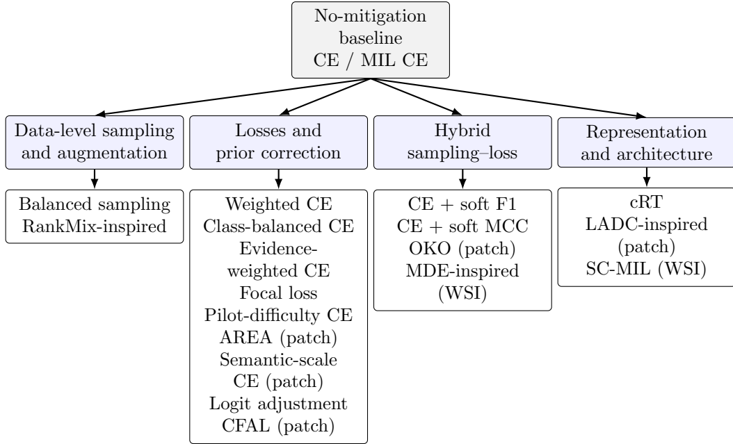
Figure 1: Intervention-level organization of the tested methods. Cross-entropy is the no-mitigation reference; alternatives intervene through sampling, objectives, prior correction, feature mixing, feature synthesis, or representation and classifier design. Table 2 adds the orthogonal signal axis.
