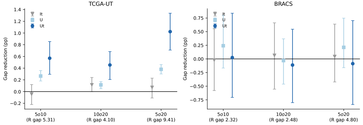
Figure 1: Only the patient-covariance loss narrows the patient-count gap, and only on TCGA-UT. Paired reduction of the real patient-count gap in percentage points, for each step between patient counts; the real gap is given below each step. Error bars show the paired 95% bootstrap intervals.
