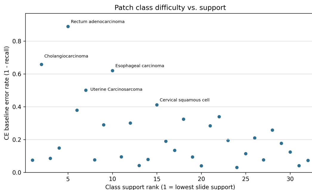
Figure 9: Patch CE-baseline class error rate versus full-dataset class-support rank. The hardest patch classes are not simply ordered by rarity, indicating that exposure-based corrections address only part of the error pattern.
