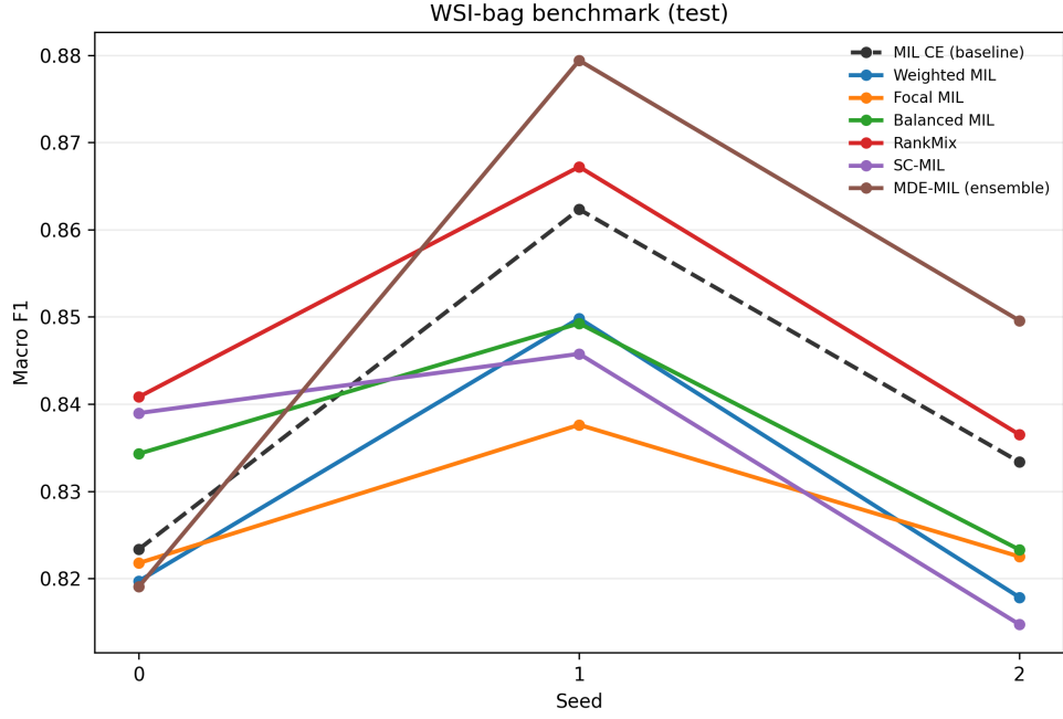
Figure 7: Primary-protocol WSI-bag macro F1 on the held-out test split by random seed. The dashed line marks plain MIL CE; seed-wise spread shows why cross-method gaps should be read cautiously when standard deviations overlap (Table 7).
