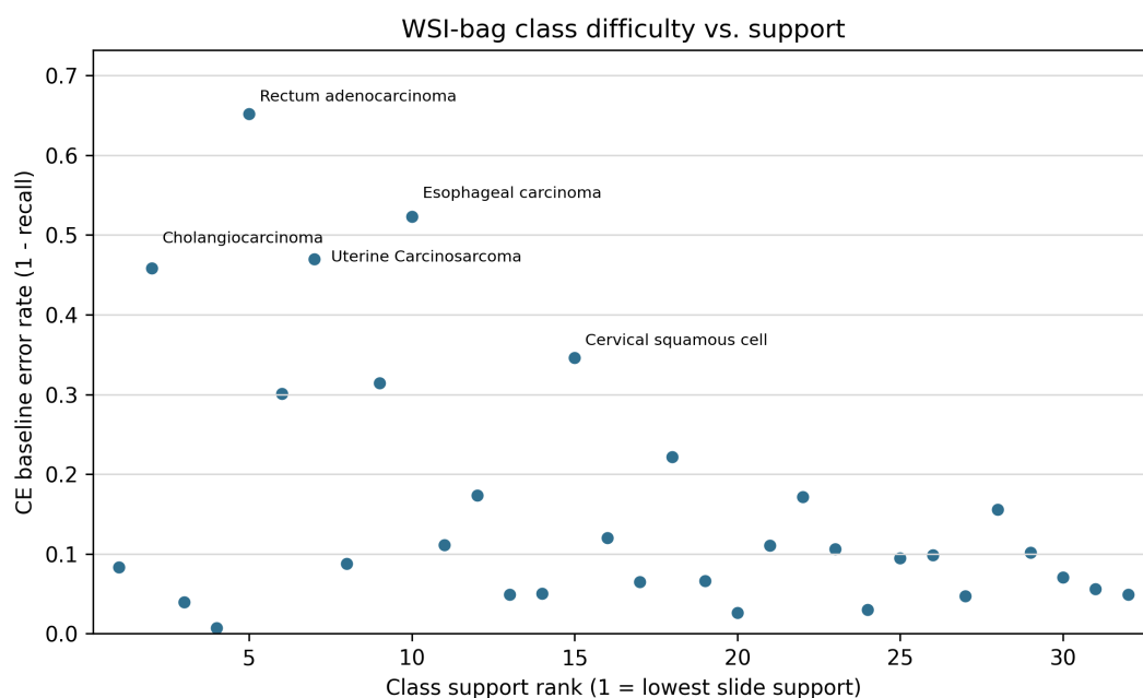
Figure 10: WSI-bag CE-baseline class error rate versus full-dataset class-support rank. The same high-error classes are visible at slide level, showing that class difficulty is not reducible to class frequency.
