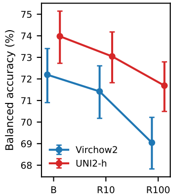
TCGA-UT
