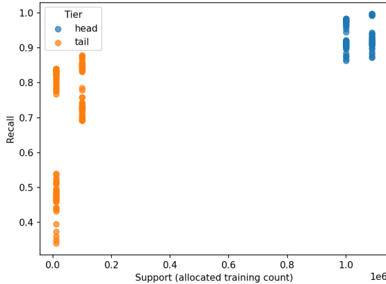
(c) PANDA
