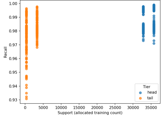
(b) CAMELYON16
