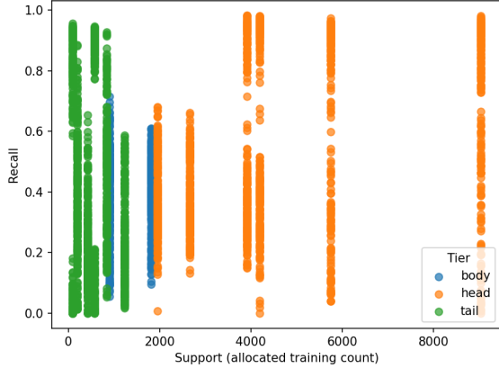
(a) BRACS
