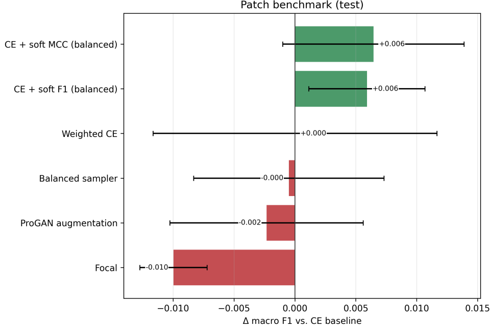
Figure 4: Patch-level change in macro F1 relative to the CE baseline on the held-out test split. Bars show the mean \Delta over seeds 0–2 with seed-wise standard deviation. Positive values indicate improvement over CE; near-zero values indicate no meaningful mean change. Values should only be interpreted within the patch benchmark (Table 5).
