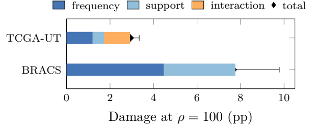
Figure 3: Damage at \rho = 100 by component; diamonds give the total with its 95% interval.
