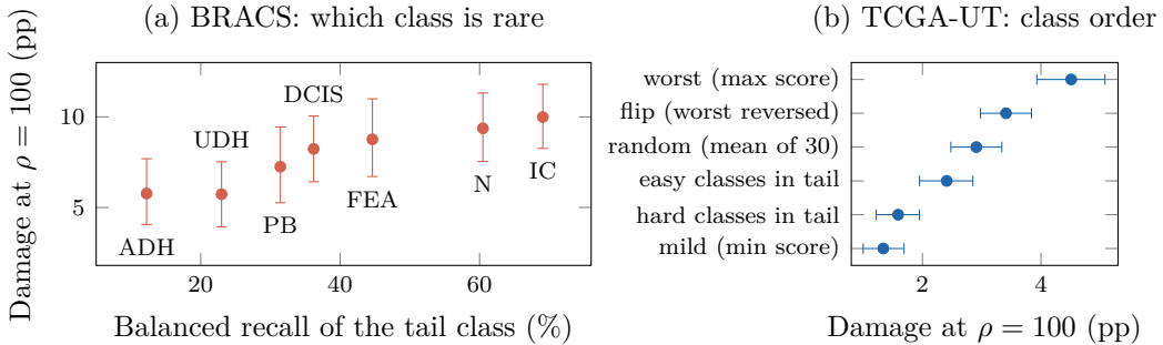
Figure 4: Damage at \rho = 100 with 95% intervals. (a) BRACS with each class in the tail in turn, against its balanced-condition recall (Spearman 0.96 , n = 7 ). (b) TCGA-UT class-to-rank assignments.
