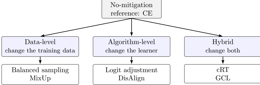
Figure 1: The six methods in the three families of Krawczyk (2016). CE on the empirical distribution is the no-mitigation reference.
