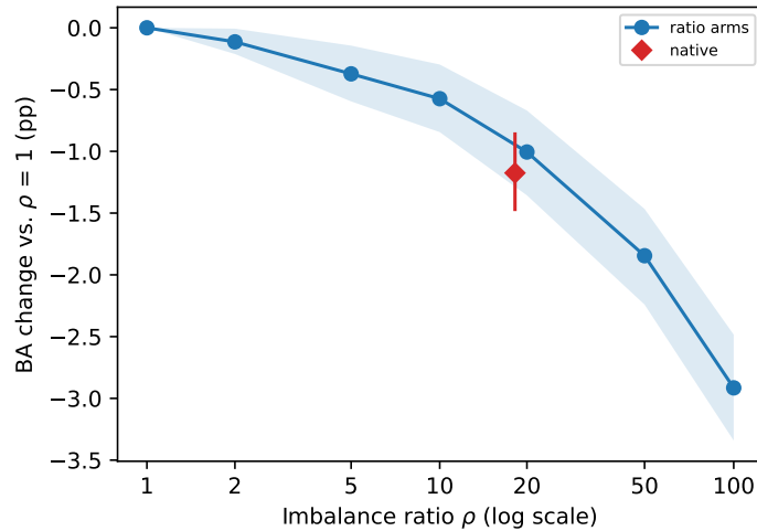
Figure 1: Balanced accuracy degrades slowly and accelerates beyond \rho = 10 . The line shows the change in patient-macro balanced accuracy relative to the balanced arm, with the ratio arms at their realized ratio and a shaded paired 95% bootstrap band; the red diamond marks the native allocation at its realized ratio of 18.1.
