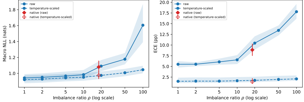
Figure 2: Raw probability quality degrades much faster than accuracy but recovers almost completely under temperature scaling. Left: macro NLL; right: ECE; both raw (solid, filled) and after validation temperature scaling (dashed, open). Blue lines connect the ratio arms at their realized ratio, with shaded paired 95% bootstrap bands; the red diamonds mark the native allocation at its realized ratio of 18.1.
