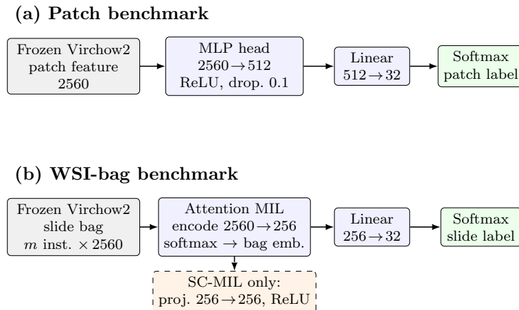
Figure 3: Shared classifier heads for the fixed training protocol. Panel (a) classifies one controlled patch embedding per forward pass. Panel (b) encodes all instances on a slide, pools them with attention, and predicts one slide-level label; the dashed branch is used only by SC-MIL. Virchow2 features are frozen in both benchmarks.
