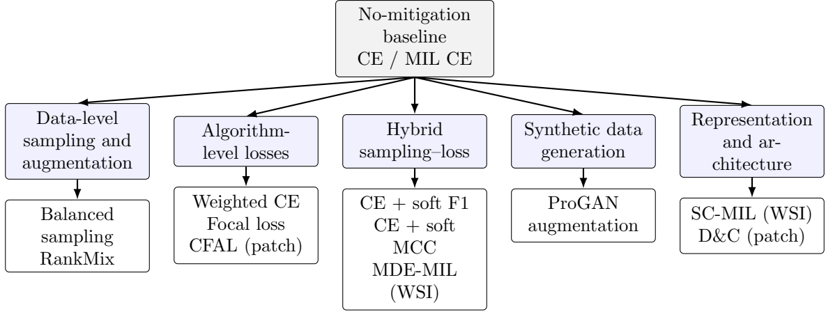
Figure 2: Method organization used in the benchmark. Cross-entropy is the no-mitigation reference, while the tested alternatives intervene through sampling, loss design, synthetic data, WSI feature augmentation, or representation learning.
