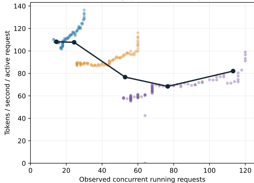
Decode throughput per active request
