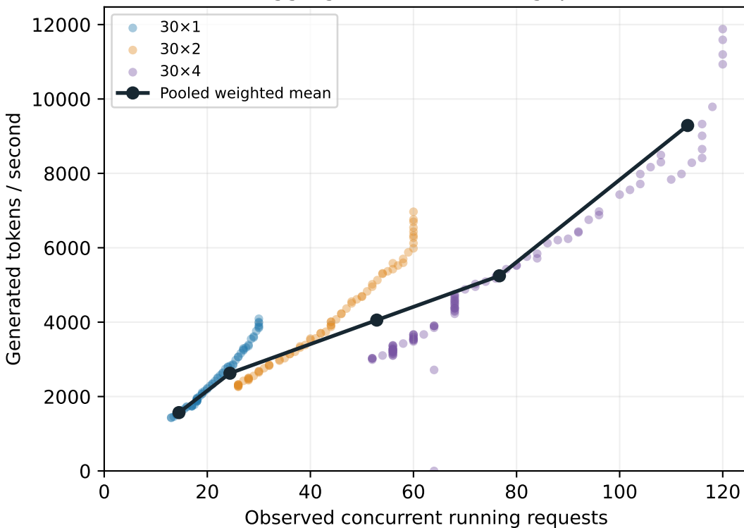
Aggregate decode throughput
