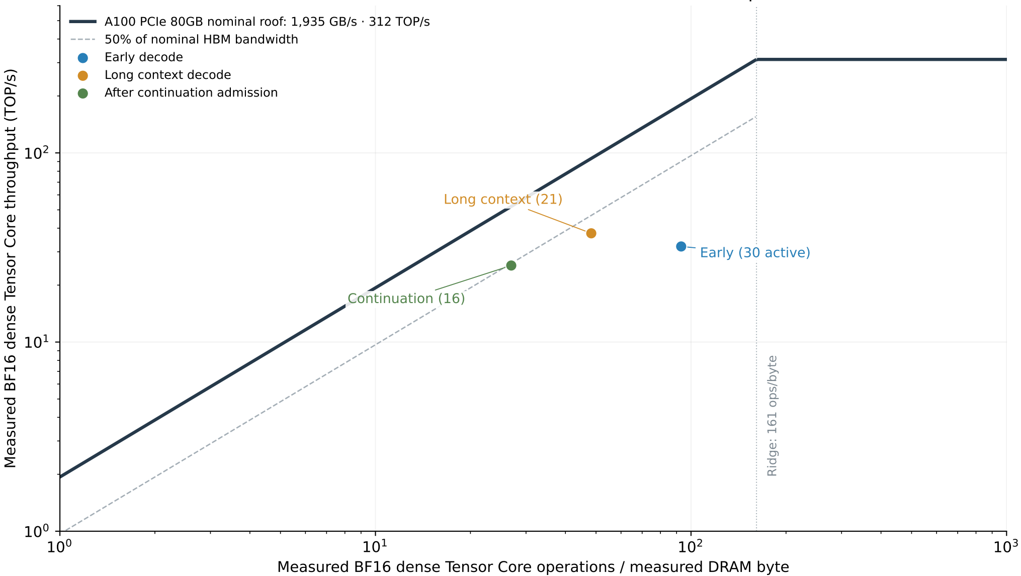
Core v1 decode on the A100: measured roofline samples
