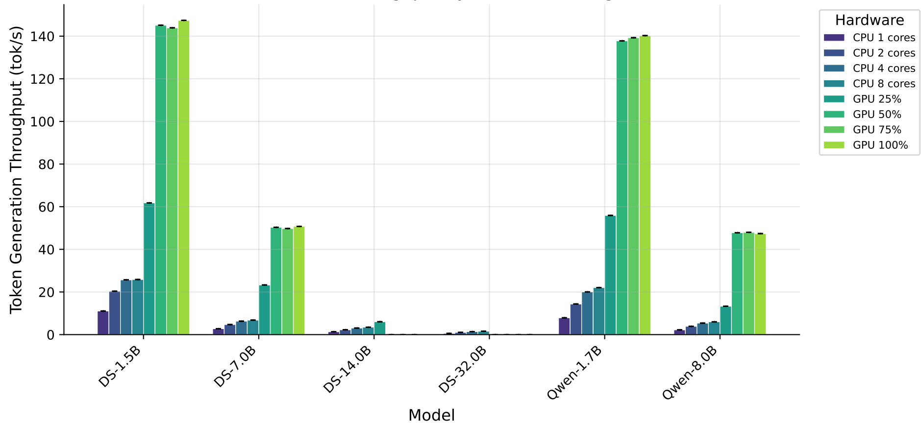
Token Generation Throughput by Hardware Configuration
