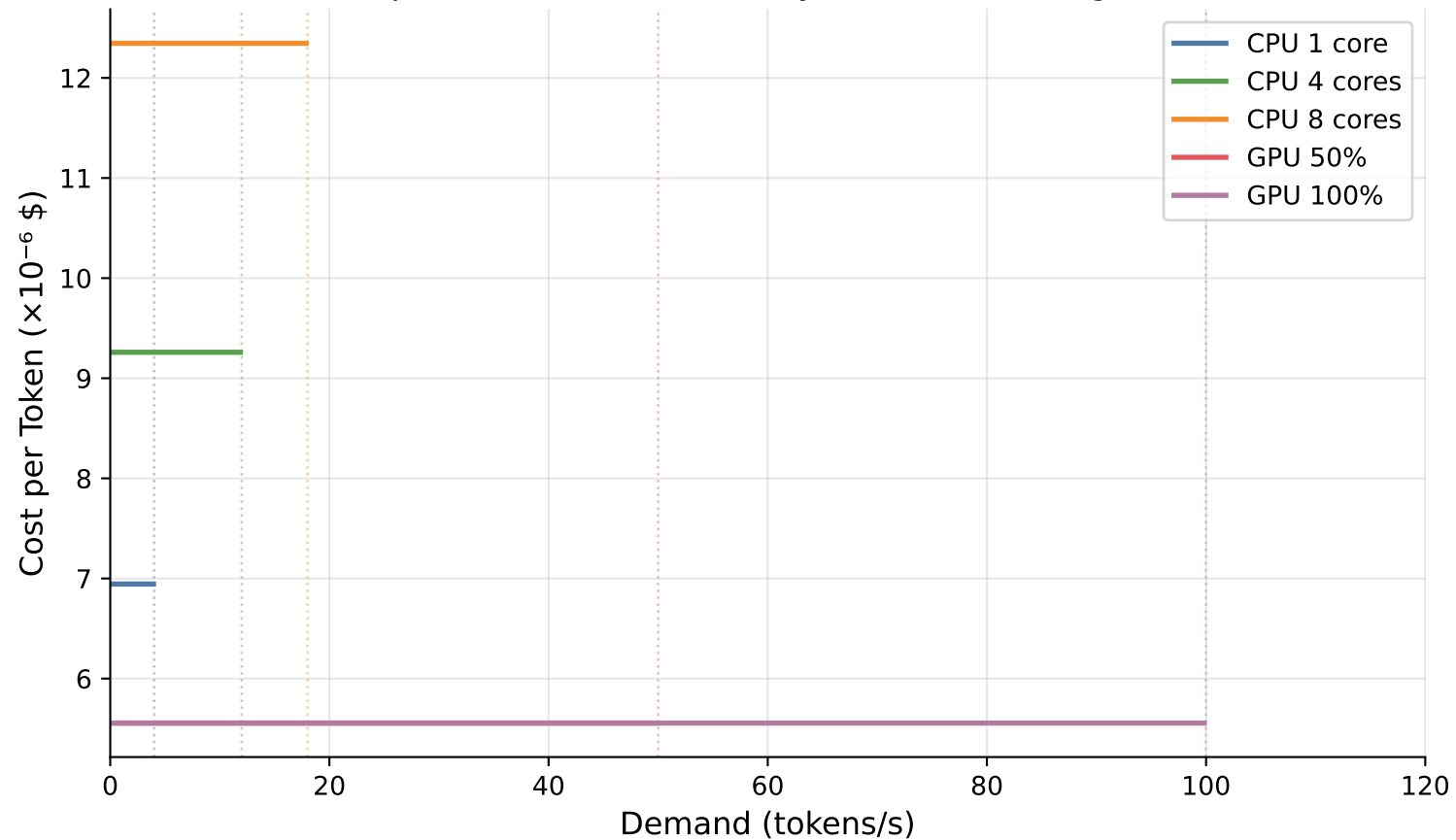
Cost per Token vs. Demand by Hardware Configuration
