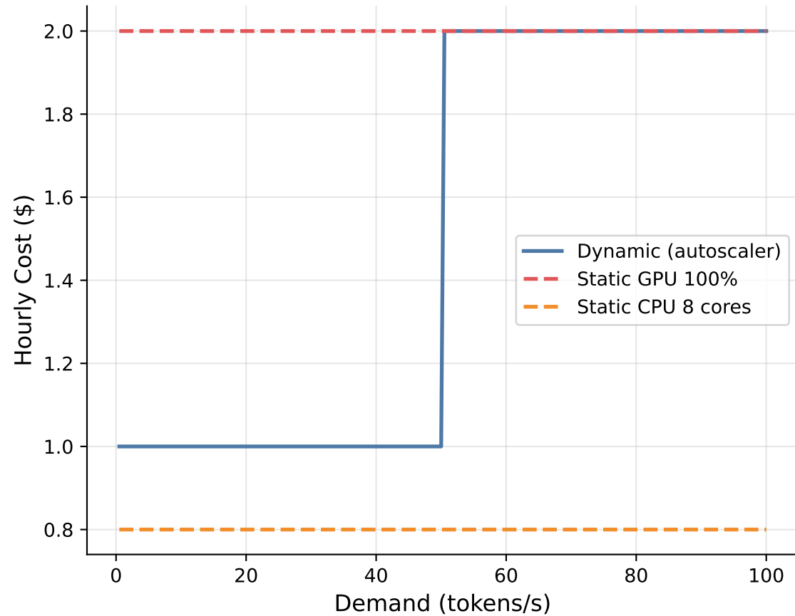
Hourly Cost: Dynamic vs. Static Allocation
