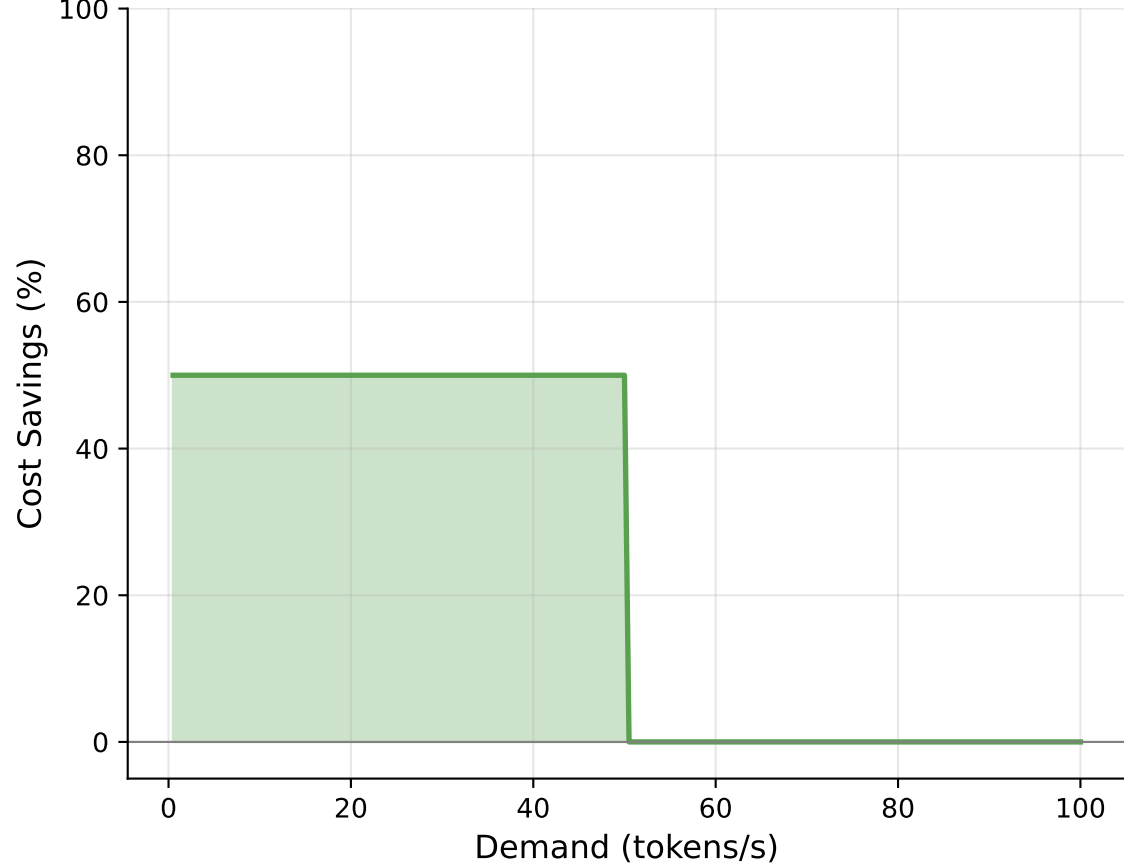
Cost Savings vs. Static GPU 100% Allocation
