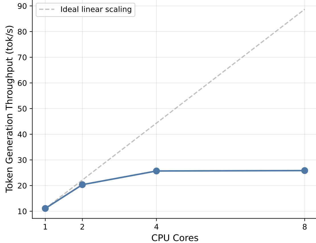
CPU Scaling: DeepSeek-R1 1.5B Q4_K_M
