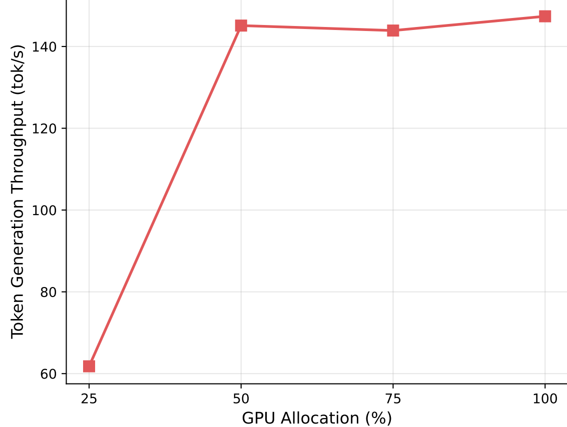
GPU Scaling: DeepSeek-R1 1.5B Q4_K_M
