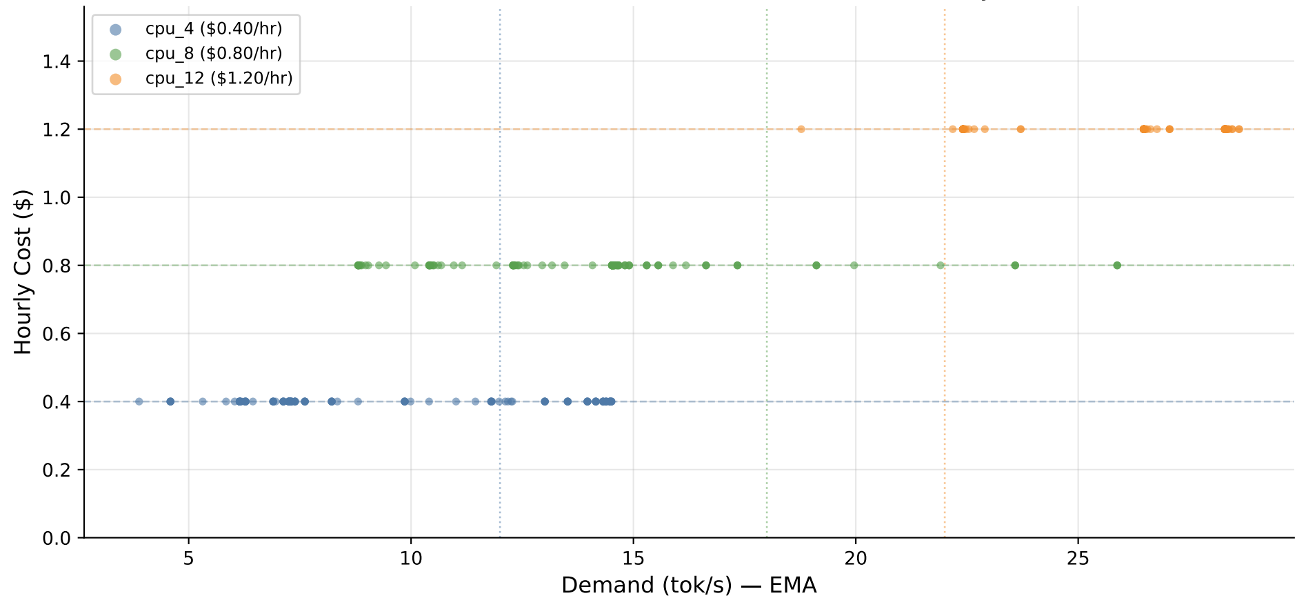
Infrastructure Cost vs. Workload Demand (CPU-only)
