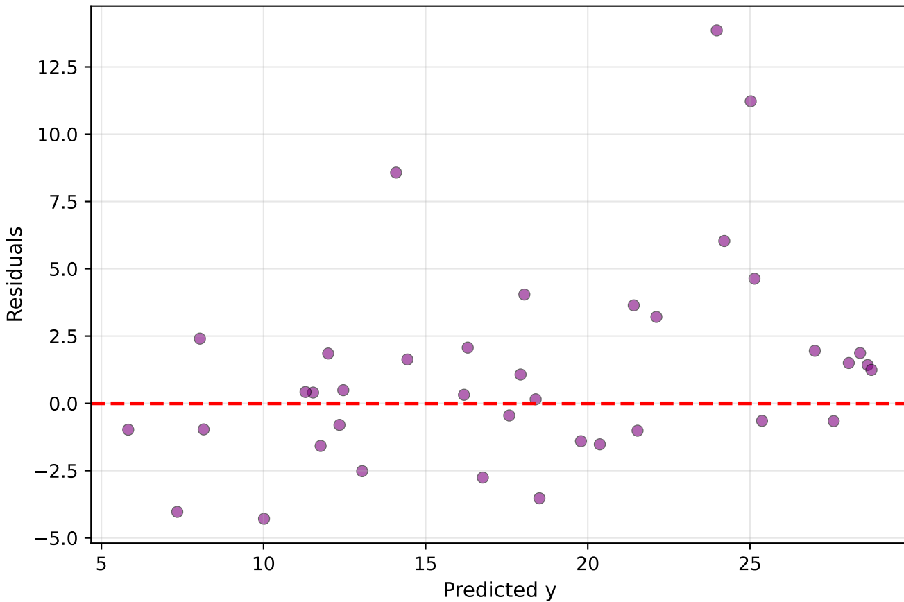
OLS Residual Plot
