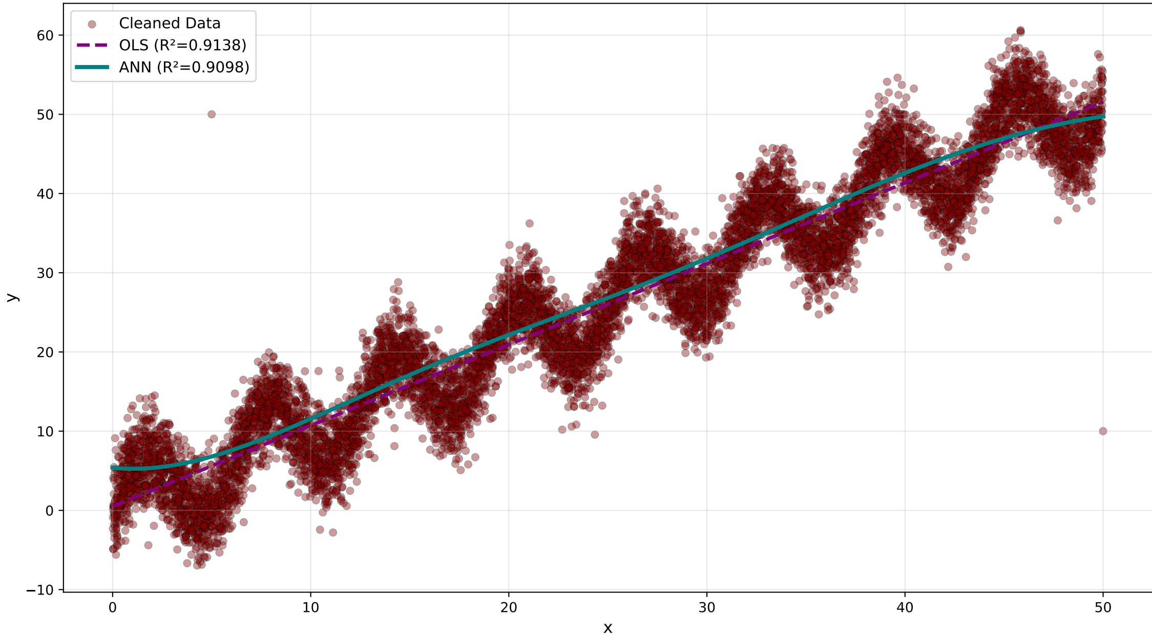
Model Comparison: OLS vs ANN (Scraped & Cleaned Data)
