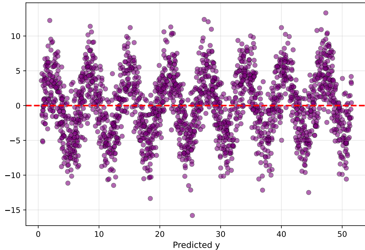
OLS Residual Plot
