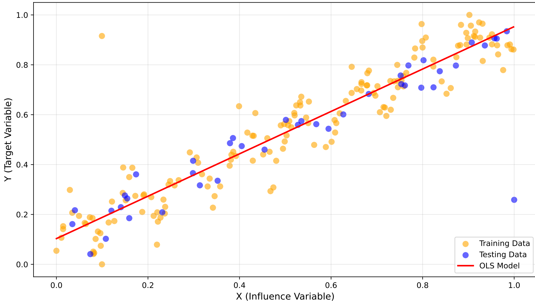
Scatter Plot with OLS Model Line
