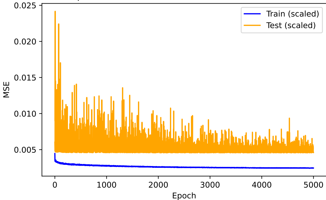
Optimized ANN (Tanh, 10 neurons) - Scaled MSE
