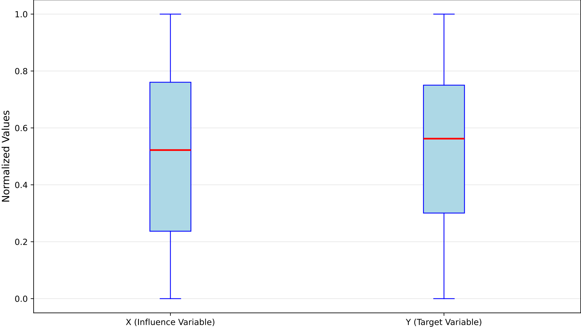
Box Plot of All Data Dimensions
