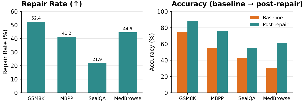
Figure 2. Left: Repair rate across benchmarks, measured as the percentage of failed execution traces converted to successful outcomes via graph-consistent counterfactual intervention. Right: Baseline versus deploy-time post-repair accuracy after applying CausalFlow without parameter updates. Improvements across all domains indicate that a substantial fraction of agent errors are attributable to localized, causally responsible steps.
