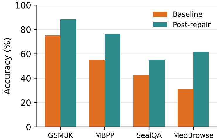
Accuracy (baseline → post-repair)
