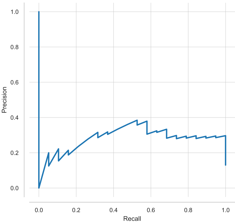
Precision-Recall Curve - RF
