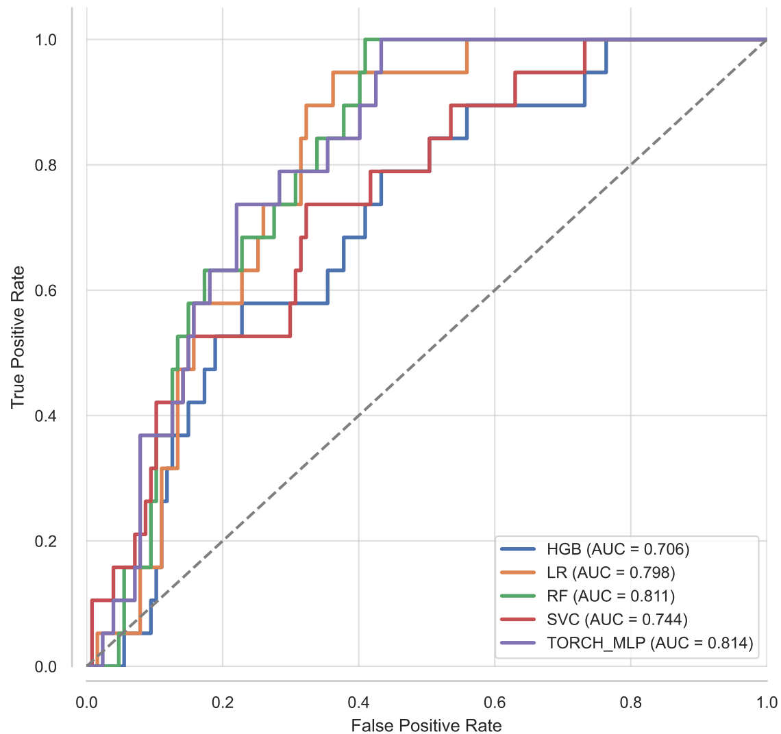
Combined ROC Curve (complications_30d)
