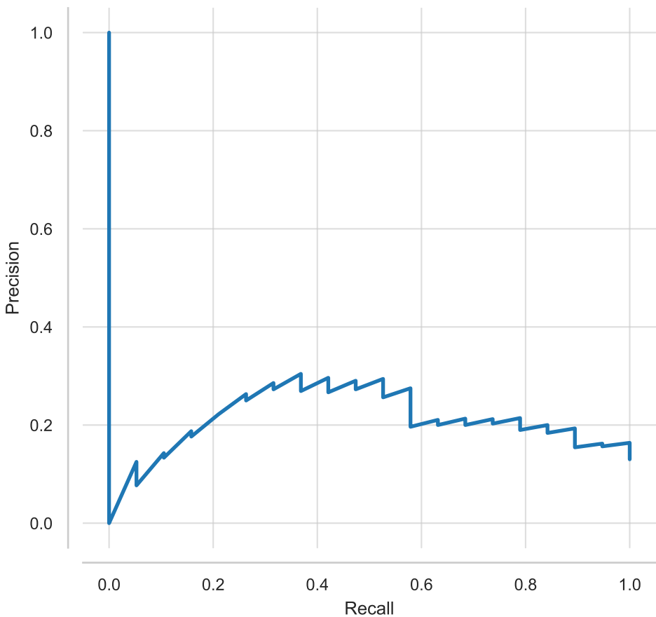
Precision-Recall Curve - HGB
