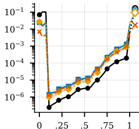
Qwen3-Embedding-0.6B
