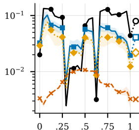
Qwen3.5-0.8B-Base
