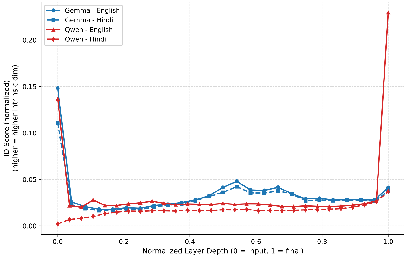
ID Score (normalized) across Layer Depth
